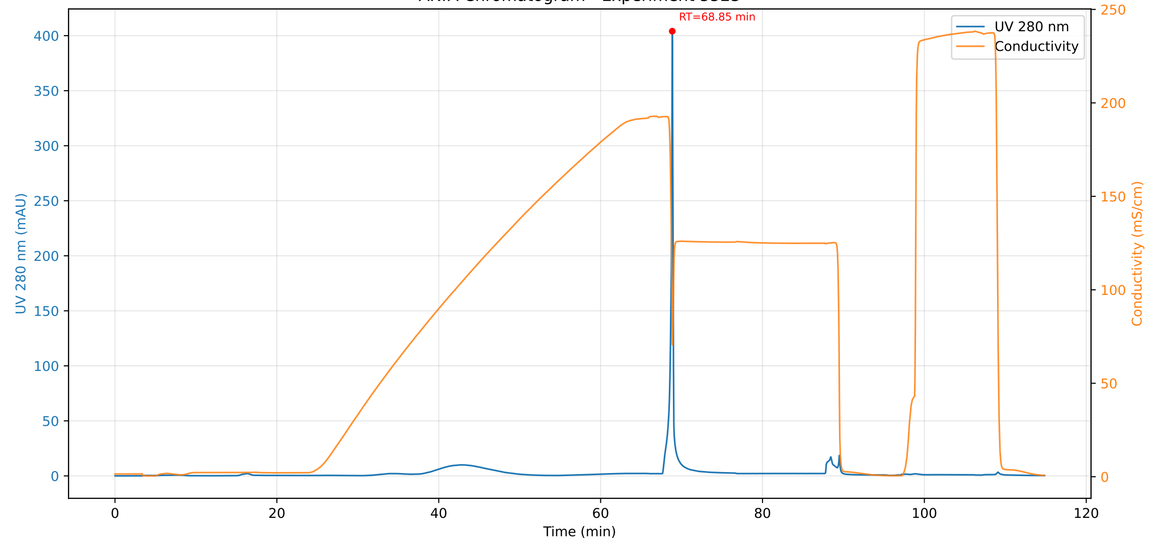
AKTA Chromatogram - Experiment 5523
